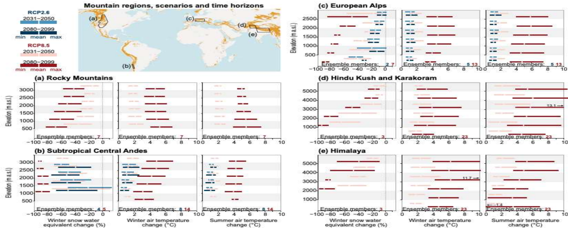
Figure 2.3 | Projected change (1986–2005 to 2031–2050 and 2080–2099) of mean winter (December to May; June to August in Subtropical Central Andes) snow water equivalent, winter air temperature and summer air temperature (June to August; December to February in Subtropical Central Andes) in five high mountain regions for RCP8.5 (all regions) and RCP2.6 (European Alps and Subtropical Central Andes). Changes are averaged over 500 m (a,b,c) and 1,000 m (d,e) elevation bands. The
