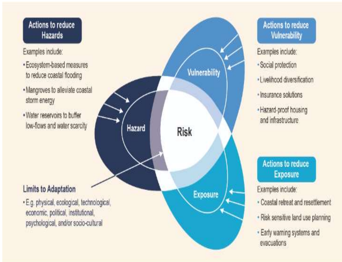
Figure TS.4 | There are options for risk reduction through adaptation. Adaptation can reduce risk by addressing one or more of the three risk factors: vulnerability, exposure, and/or hazard. The reduction of vulnerability, exposure, and/or hazard potential can be achieved through different policy and action choices over time until limits to adaptation might be reached. The figure builds on the conceptual framework of risk used in AR5 (for more details see Cross-Chapter Box 2 in Chapter 1).
